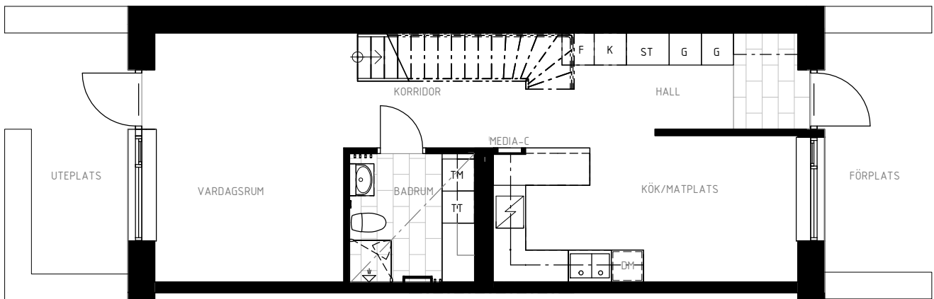
PLAN 1
