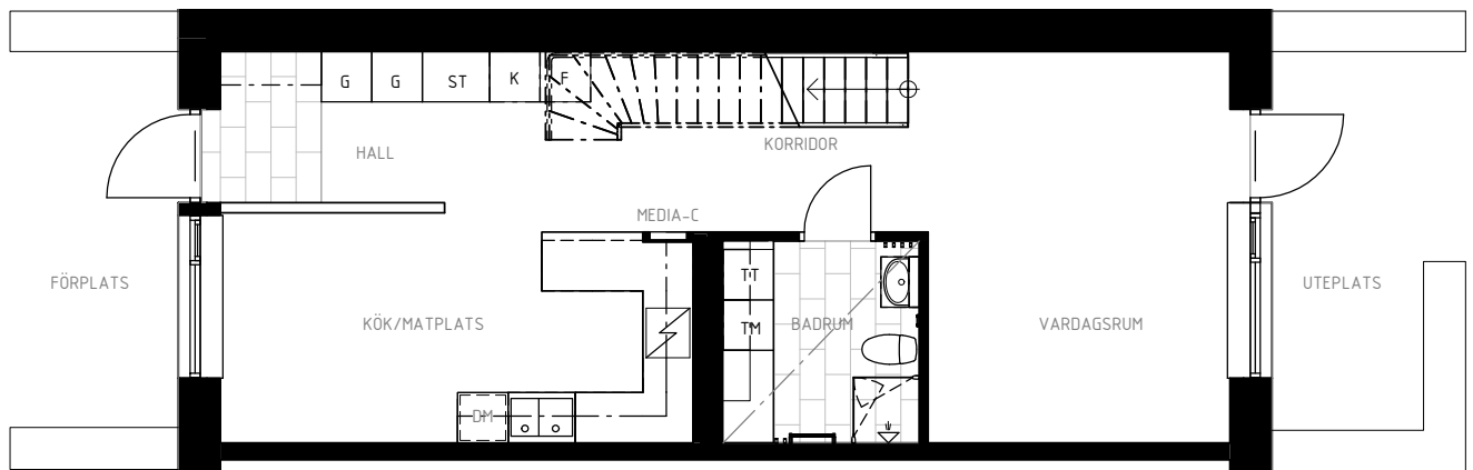
PLAN 1
